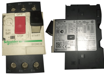
Guardamotor Regulable 13-18A Schneider Electric GV2ME20
