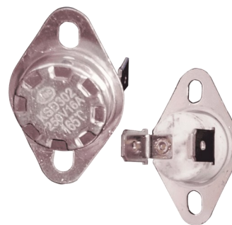
Termostato 165°C 16A 250V KSD302 NC
