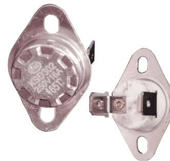
Termostato 165°C 16A 250V KSD302 NC
