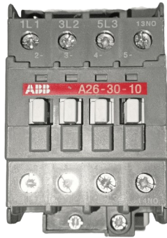
Contactor A26-30-10 110V 50Hz / 110-120V 60Hz 1SBL241001R8410
